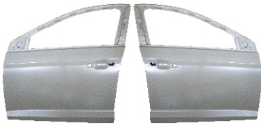
前门 FRONT DOOR-L/R L:A13/J15-6101010-DY R:A13/J15-6101020-DY
